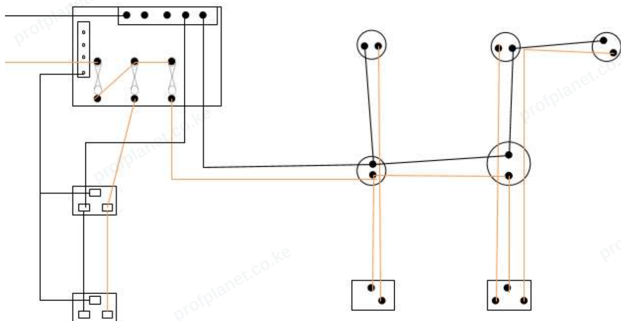
Figure 1: Wiring Diagram
