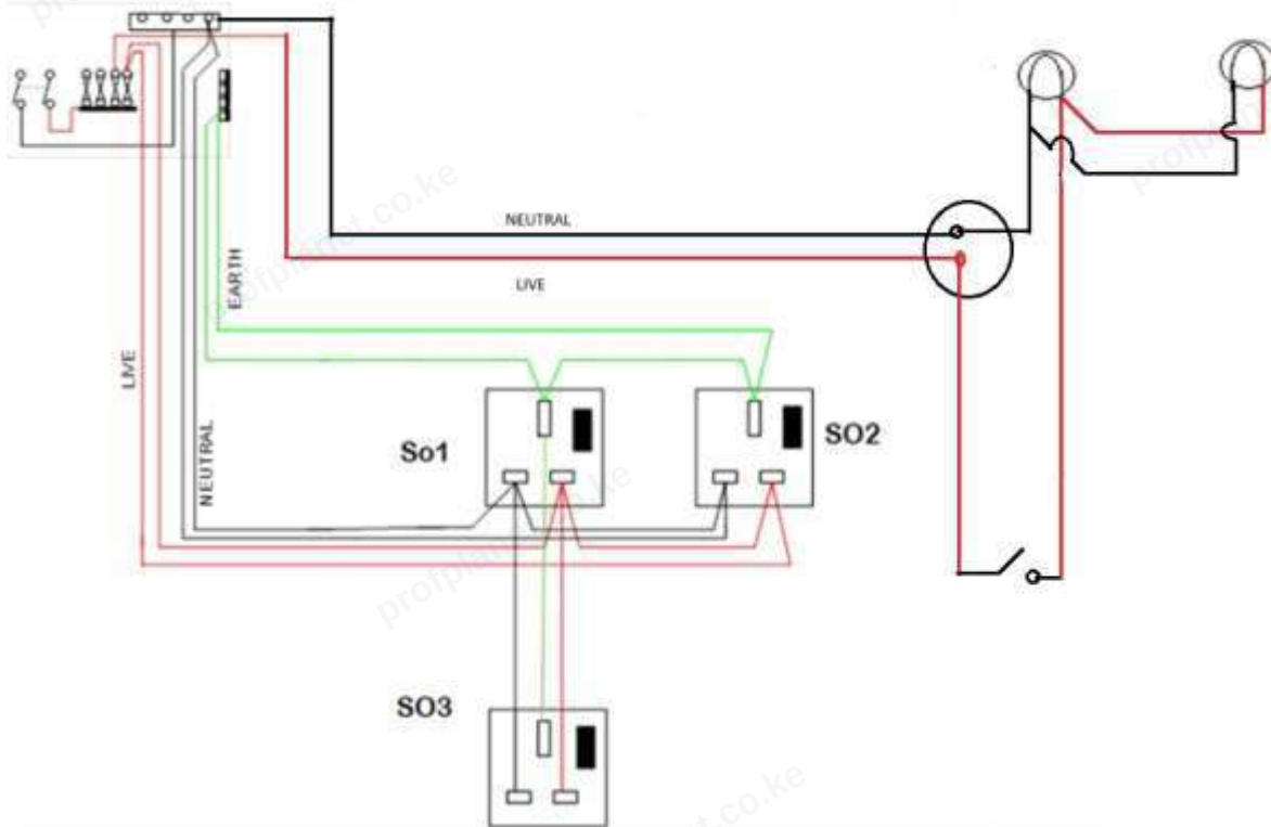
Fig 2. Wiring diagram for the two final circuits
